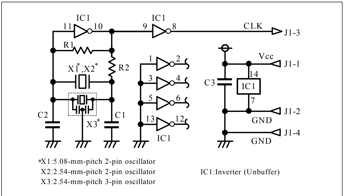
Figure 2.20 Circuit of the oscillator board OSC-2 (bare board)
